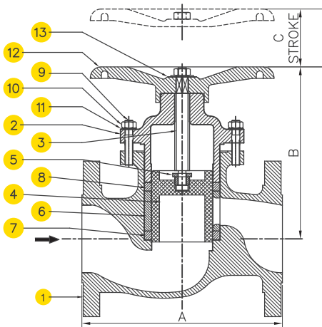
FIG. - DN80~DN150 (UNBALANCED)
